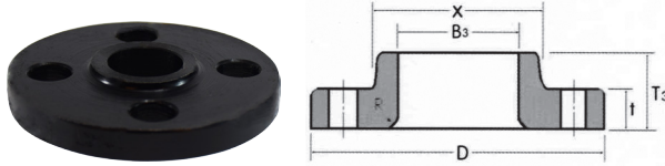
SLIP-ON 1/16" RAISED FACE FORGED STEEL FLANGE
