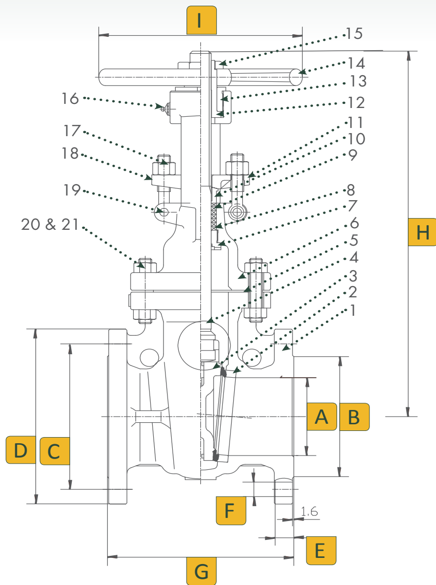
Dimensions (Inches)
