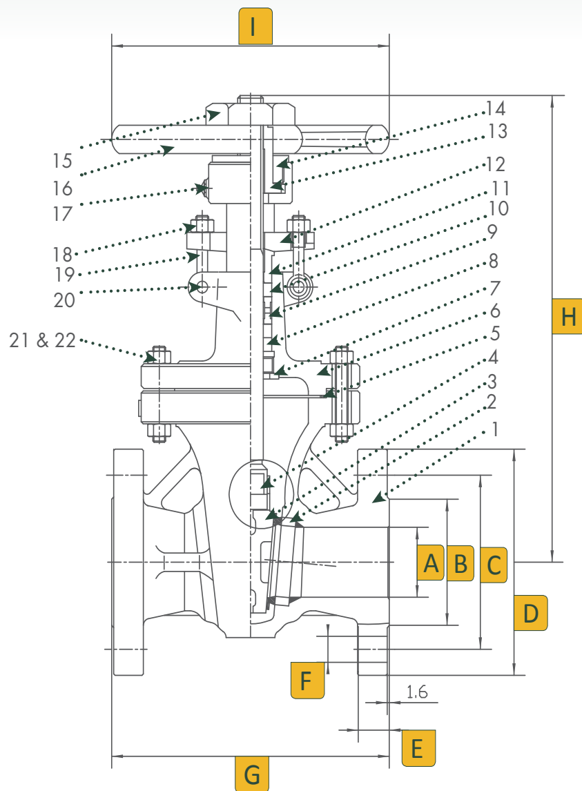
Dimensions (Inches)
