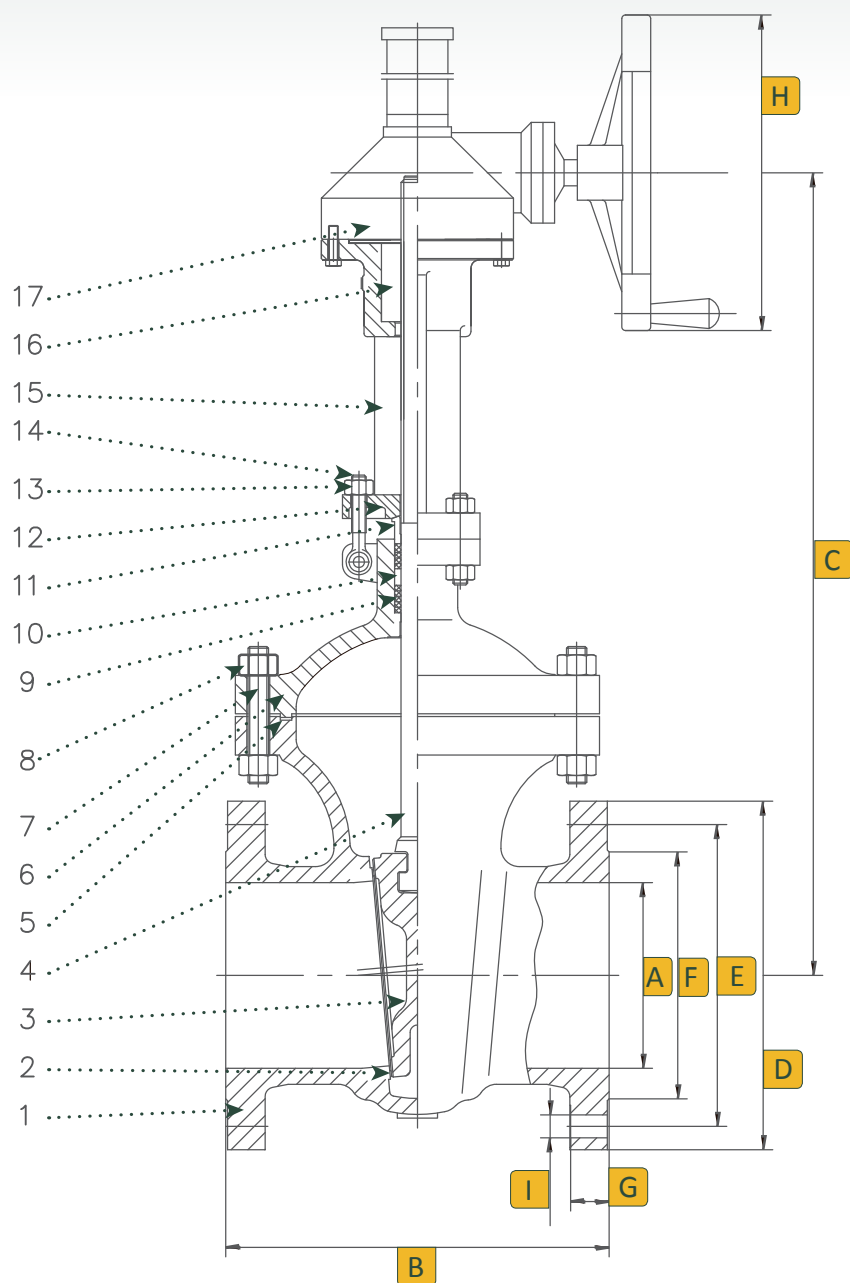
Dimensions (Inches)
